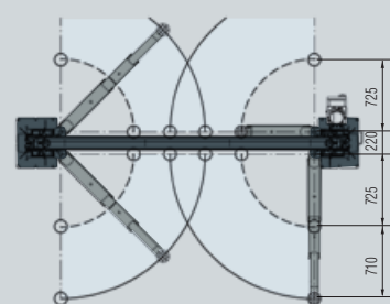
SDH370.42LIK - SDH370.45LIKEX - SDH370.50LIK
