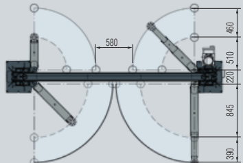
SDH370.42LIK - SDH370.45LIKEX - SDH370.50LIK
